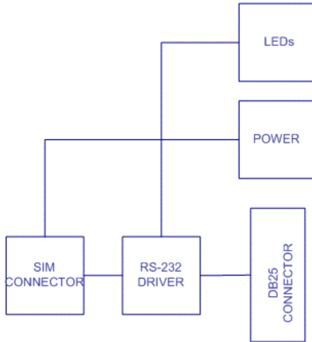
Block Diagram for the SocketModem GSM/GPRS
