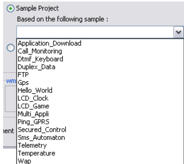
Figure 16 : Samples list
