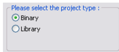
Figure 12 : Project type
