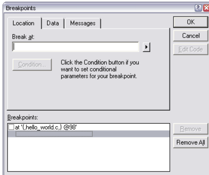
Figure 29 : Breakpoints window
